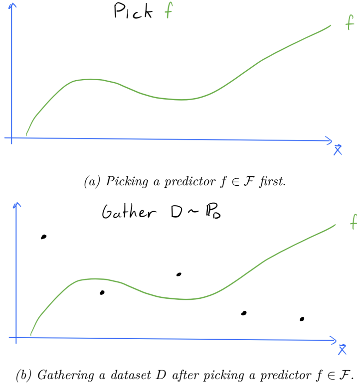
Figure 7.1: Picking a predictor f independent of the dataset D .
