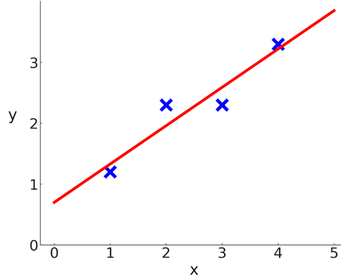
Figure 1.1: An example of a linear function fit to the dataset \mathcal{D} = \{(1, 1.2), (2, 2.3), (3, 2.3), (4, 3.3)\} . The x -axis represents the number of rooms, and the y -axis represents the price in hundreds of thousands.
