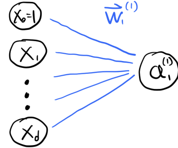
Figure 10.4: A NN representing the linear or logistic function.
