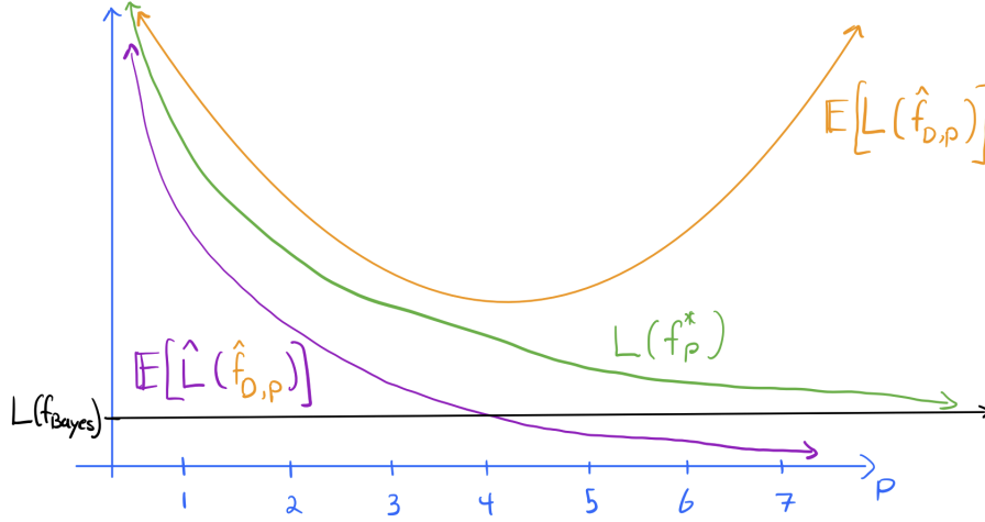
Figure 7.9: L(f_{\text{Bayes}}) , L(f_p^*) , \mathbb{E}[L(\hat{f}_{D,p})] , and \mathbb{E}[\hat{L}(\hat{f}_{D,p})] as a function of the polynomial degree p for a fixed n .
