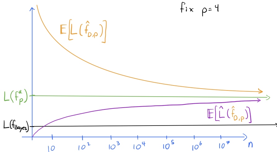
Figure 7.11: L(f_{\text{Bayes}}) , L(f_p^*) , \mathbb{E}[L(\hat{f}_{D,p})] , and \mathbb{E}[\hat{L}(\hat{f}_{D,p})] as a function of the dataset size n for a fixed p .
