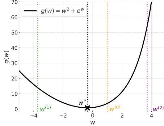
Figure 6.15: Gradient descent with large step size.
