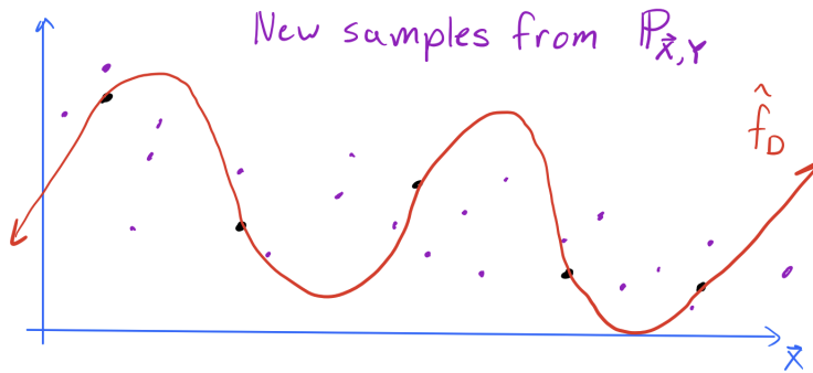
(c) Gathering new data according to \mathbb{P}_{\mathbf{X},Y} .
