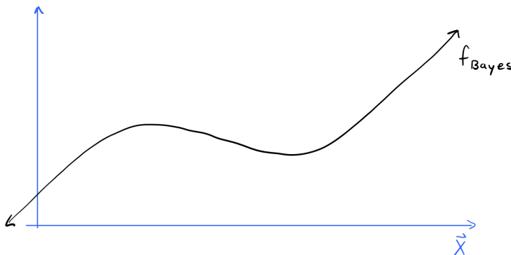
Figure 7.6: f_{\text{Bayes}} .
