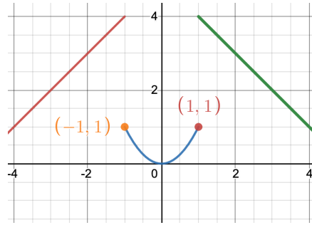
Figure 2.1: An example of a function that is not continuous, with formula in Eq. (2.1).
