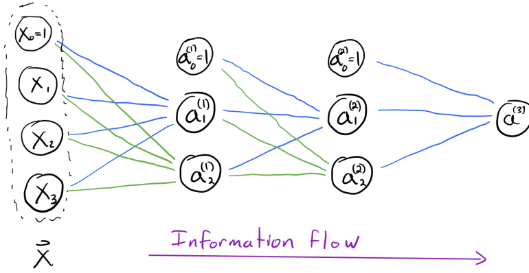
Figure 10.1: A specific neural network.
