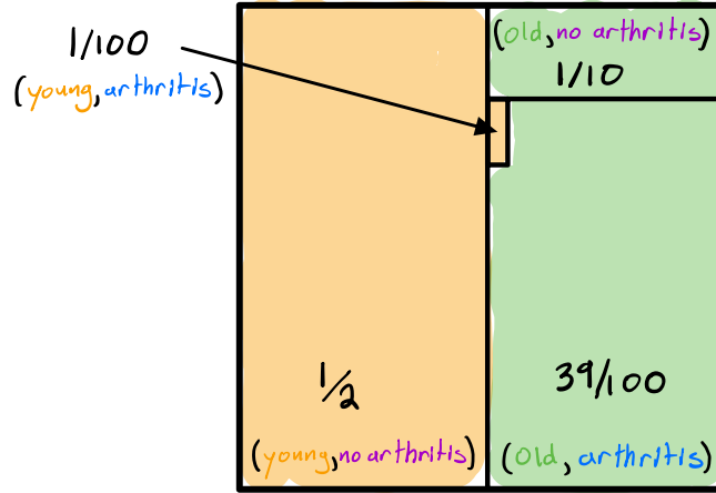
Figure 3.3: The orange area represents the value p_X(\text{young}) = \frac{51}{100} , while the green area represents the value p_X(\text{old}) = \frac{49}{100} .
