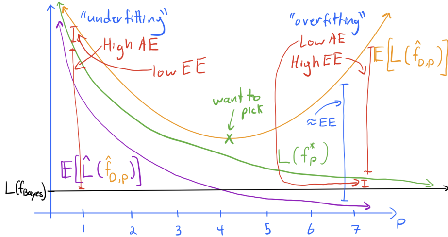
Figure 7.10: Annotated version of L(f_{\text{Bayes}}) , L(f_p^*) , \mathbb{E}[L(\hat{f}_{D,p})] , and \mathbb{E}[\hat{L}(\hat{f}_{D,p})] as a function of the polynomial degree p for a fixed n .
