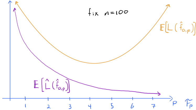
Figure 7.4: \mathbb{E}[\hat{L}(\hat{f}_{D,p})] and \mathbb{E}[L(\hat{f}_{D,p})] as a function of the polynomial degree p for a fixed dataset size n = 100 .
